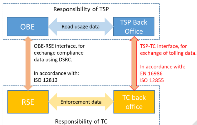
Figure 2: Interfaces in the Danish KmToll scheme
